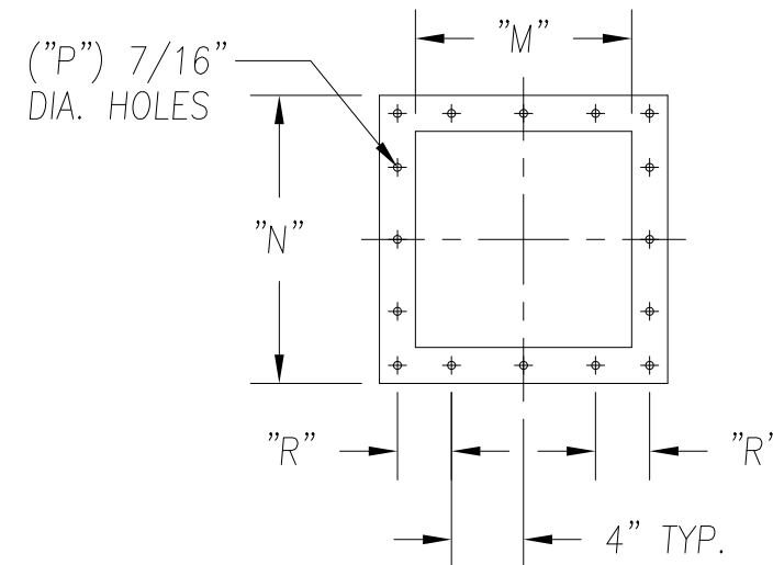
INLET/OUTLET FLANGE DETAIL
