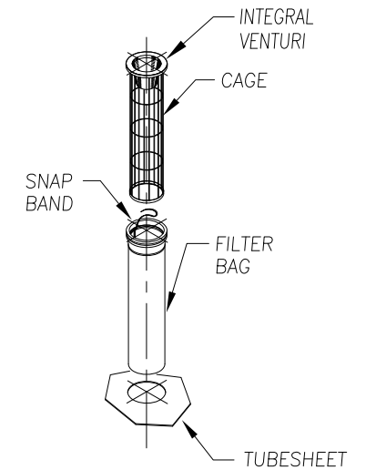
TOP REMOVAL BAG ASSEMBLY
