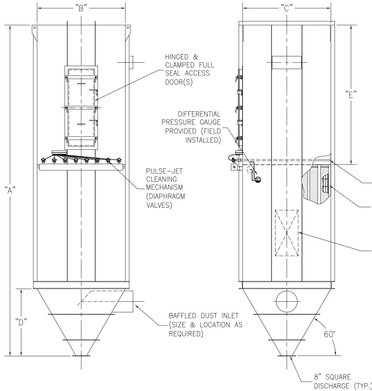
WALK-IN BAG REMOVAL DUST COLLECTOR ( 196 TO 256 BAGS )
