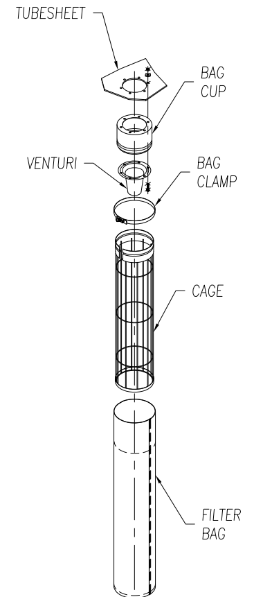
BOTTOM REMOVAL BAG ASSEMBLY
