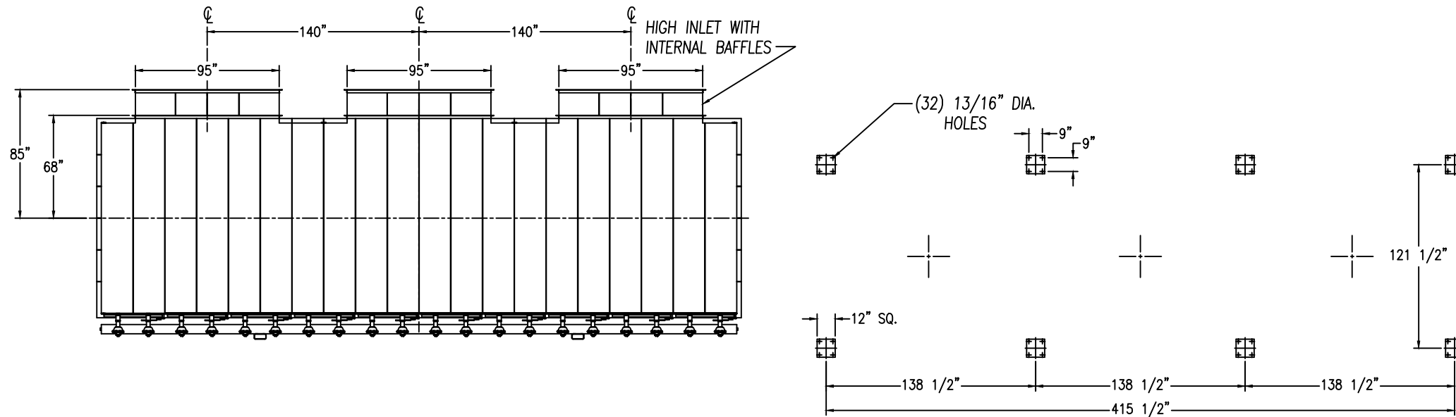
ANCHOR PLAN
