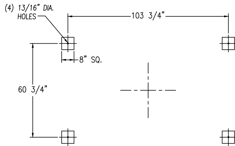
ANCHOR PLAN
