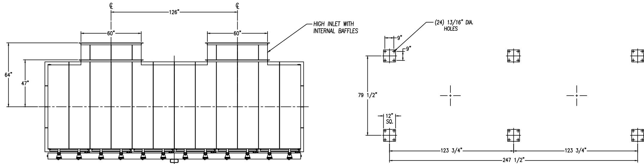
ANCHOR PLAN
