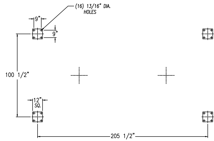
ANCHOR PLAN
