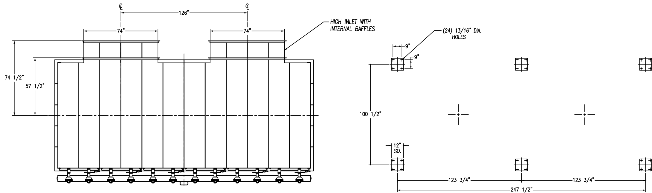
ANCHOR PLAN
