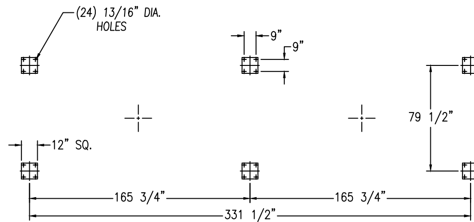
ANCHOR PLAN
