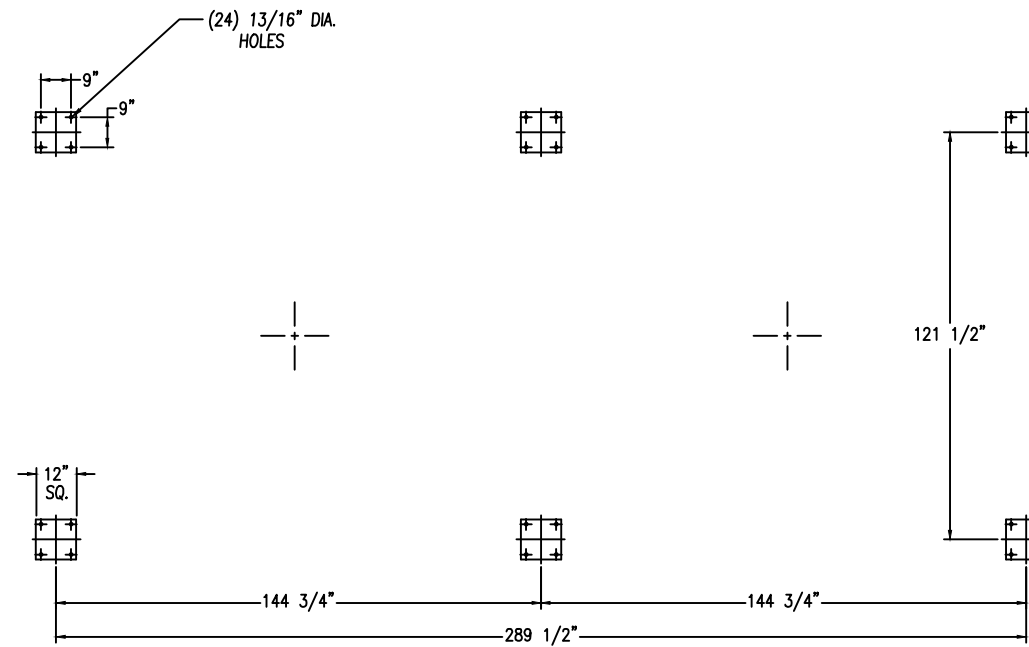
ANCHOR PLAN
