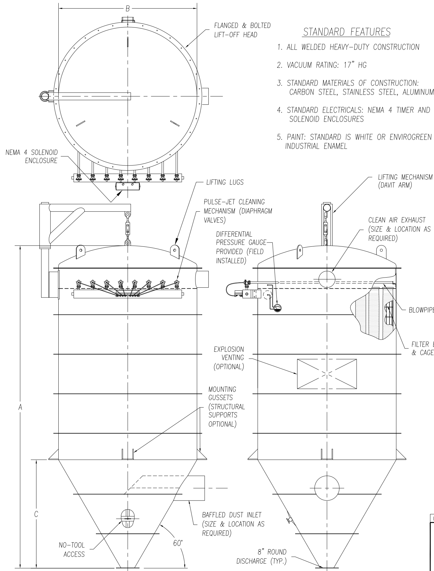
TOP REMOVAL BAG PNEUMATIC RECEIVER ( 37 TO 180 BAGS )
