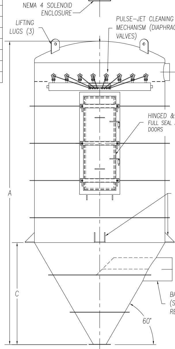
BOTTOM REMOVAL CARTRIDGE PNEUMATIC RECEIVER ( 114 TO 180 CARTRIDGES )
