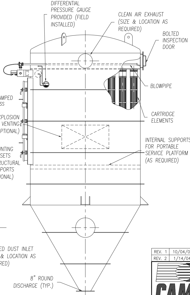
BOTTOM REMOVAL CARTRIDGE PNEUMATIC RECEIVER ( 114 TO 180 CARTRIDGES )
