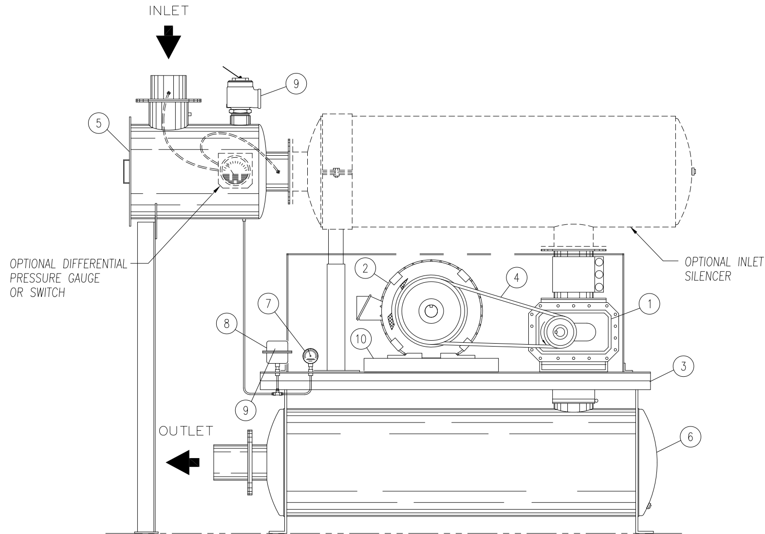
HORIZONTAL STYLE VACUUM BLOWER PACKAGE ( 3 HP TO 75 HP )
